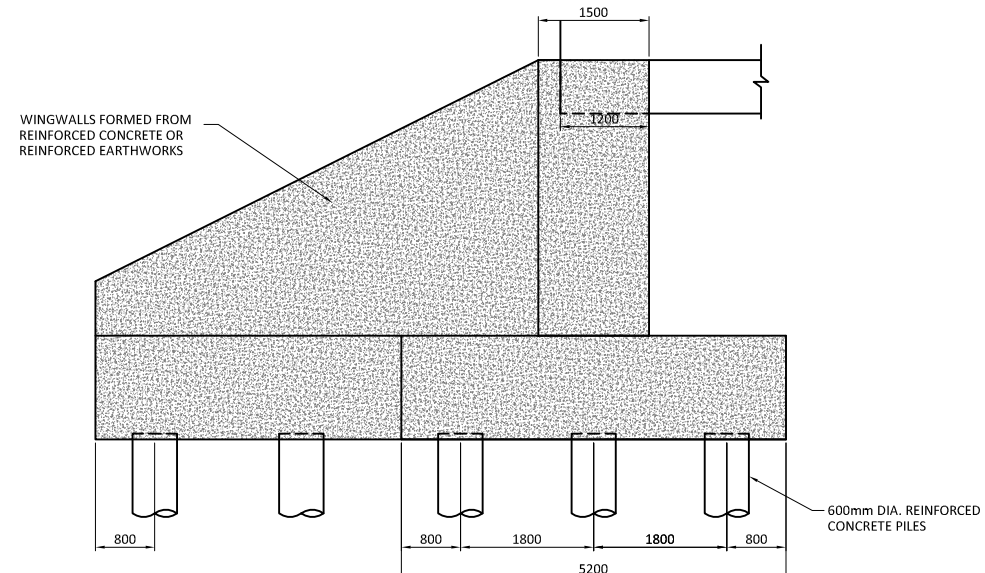
INTEGRAL ABUTMENT SCALE 1:50
